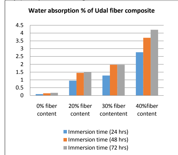
Fig.1: Water absorption %
